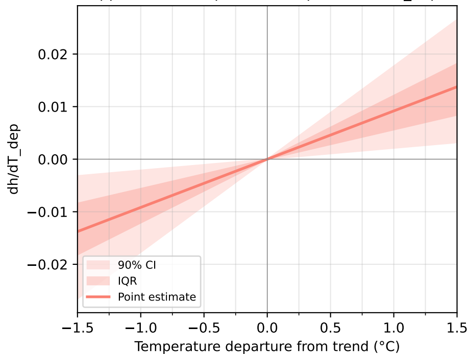
Approach 6e: Departure component ( 2h_4T_{dep} )
