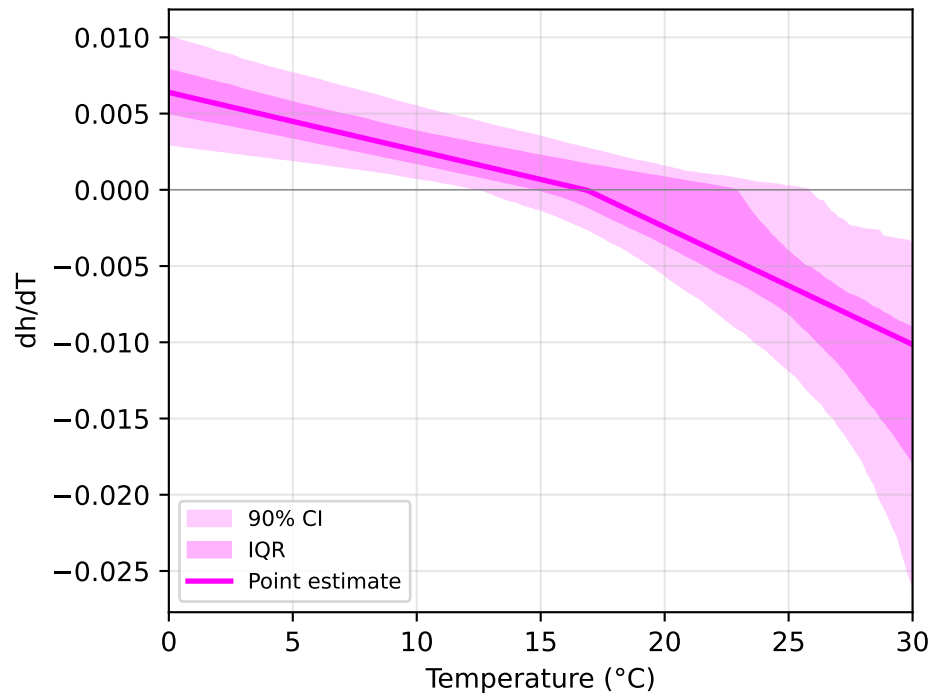
Approach 6e: Departure component ( 2h_4T_{dep} )
