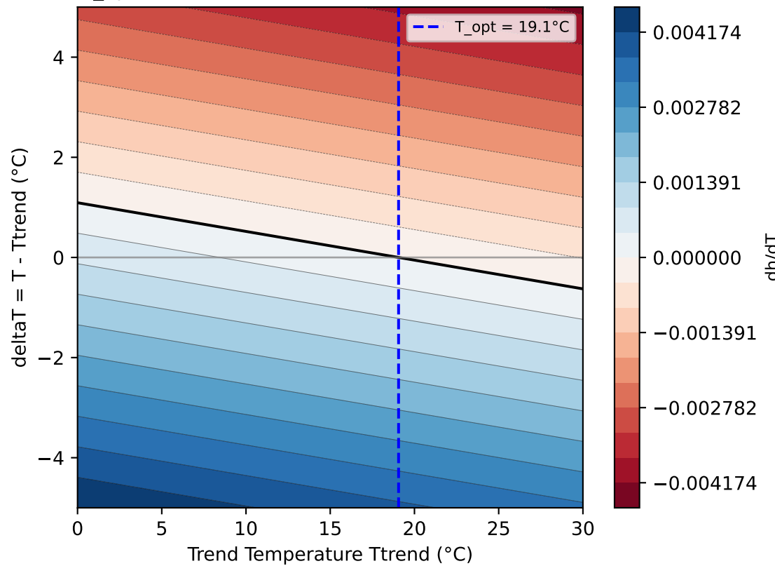
8a: Shared T_{opt} Total/Trend LOESS: Total - Trend Derivative (x= T )
