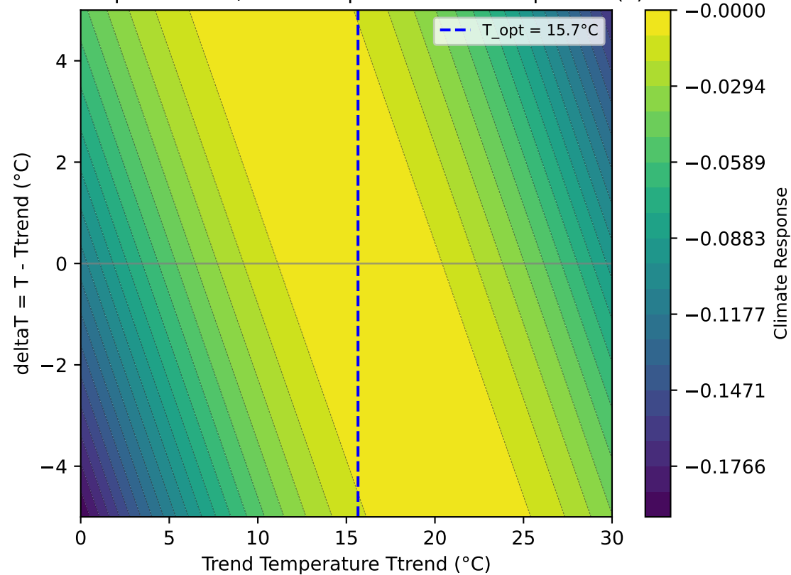
6a: Separate Total/Trend Freq LOESS: Total - Trend ( x=T_{trend} )
