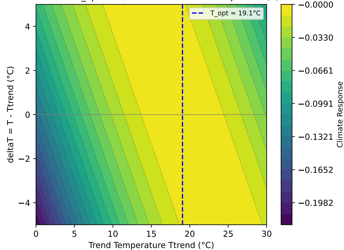
8a: Shared T_{opt} Total/Trend LOESS: Total - Trend ( x=T_{trend} )
