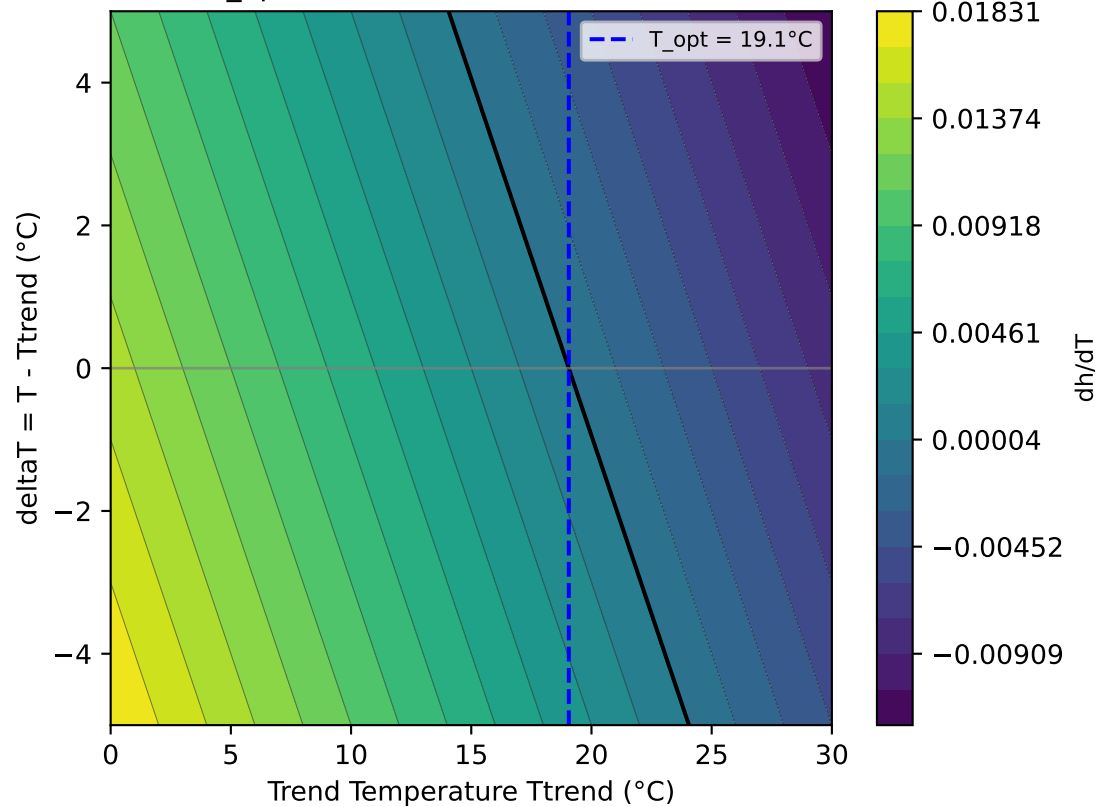
8a: Shared T_{opt} Total/Trend LOESS: Total - Trend Derivative (x= T_{trend} )
