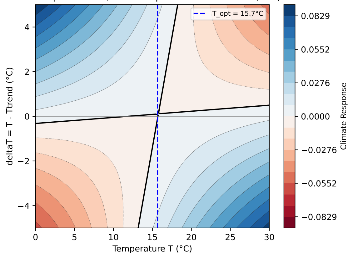
6a: Separate Total/Trend Freq LOESS: Total - Trend ( x=T )
