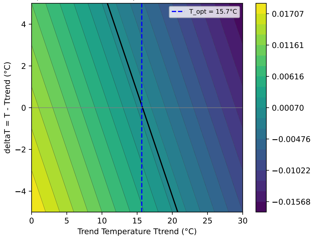
6a: Separate Total/Trend Freq LOESS: Total - Trend Derivative (x= T_{trend} )
