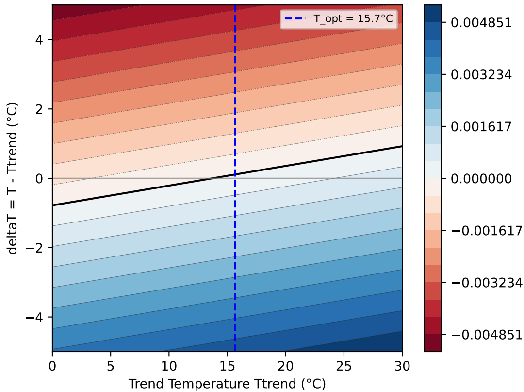
6a: Separate Total/Trend Freq LOESS: Total - Trend Derivative (x= T )
