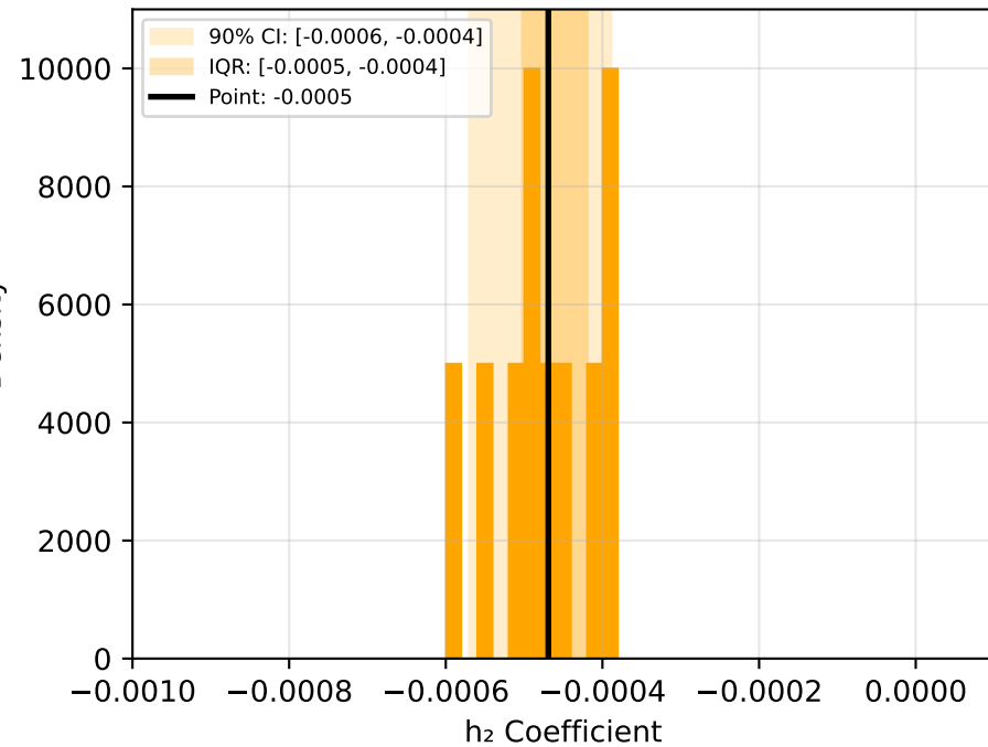
Approach 6: h_2
