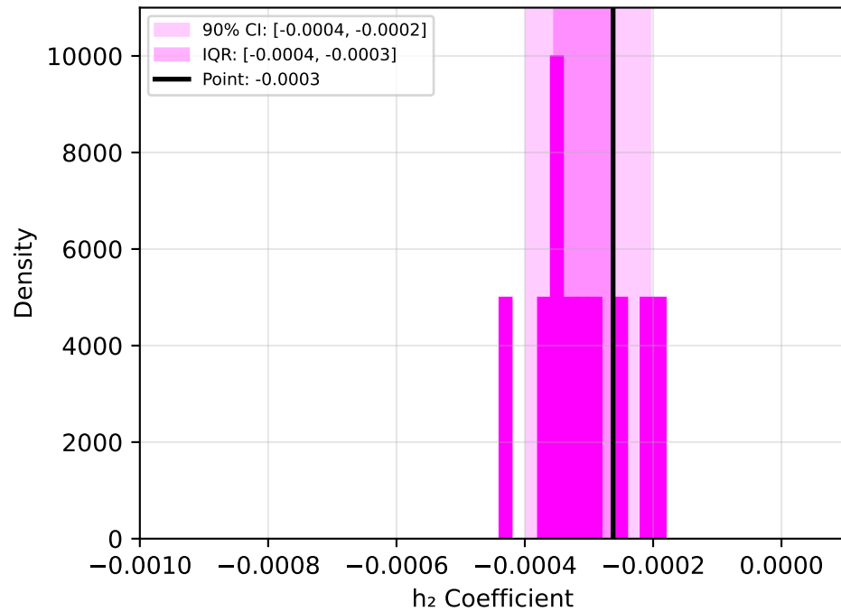
Approach 8: h_2 ( T \leq T_{\text{opt}} )
