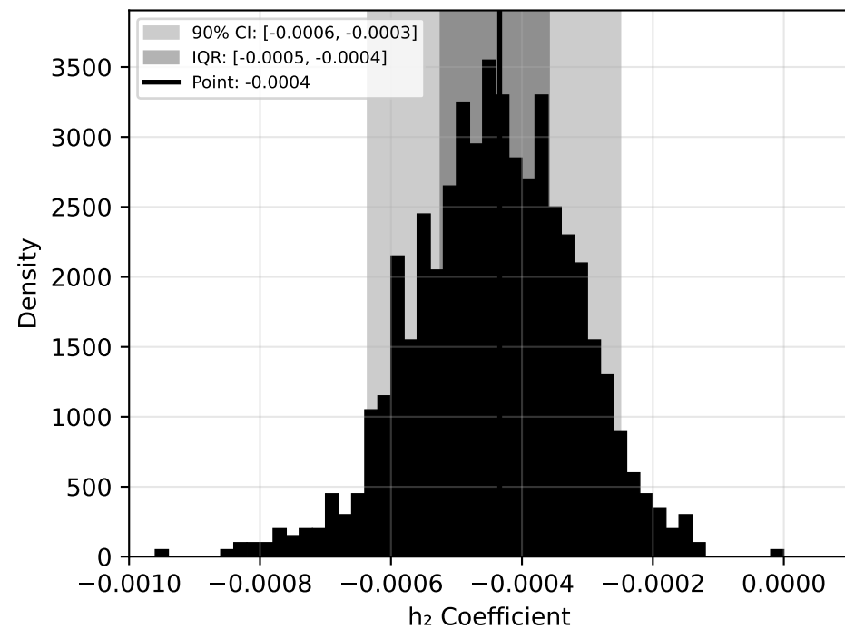
method2: h_2
