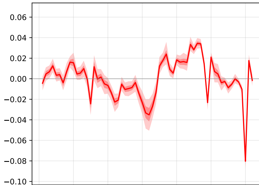
1: Combined Detrending (Mixed)
