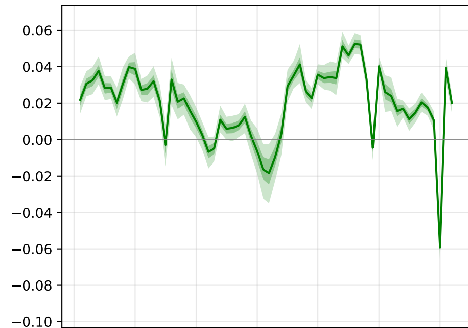
2: Linear Temperature Detrending
