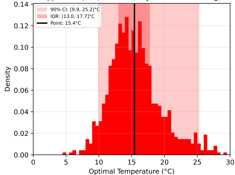
Approach PP: Piecewise (Polynomial Detrending)
