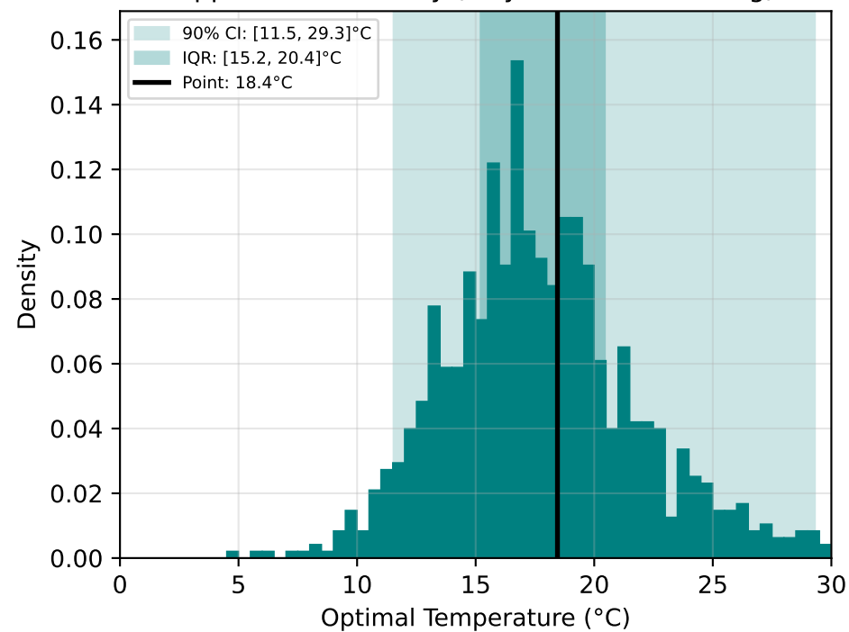
Approach DP: Decay (Polynomial Detrending)
