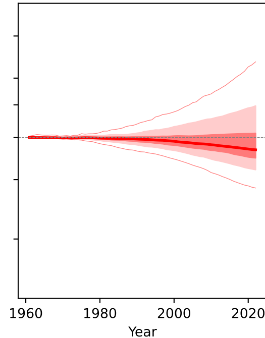
approach1
