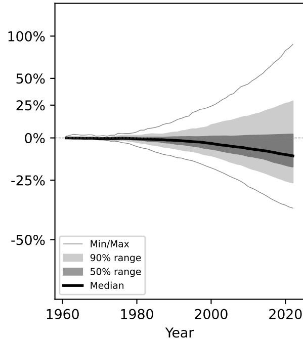
approach0
