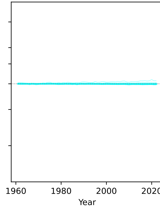
approach4
