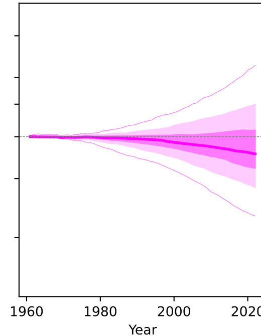
approach3
