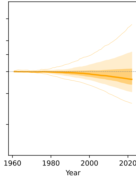
approach2
