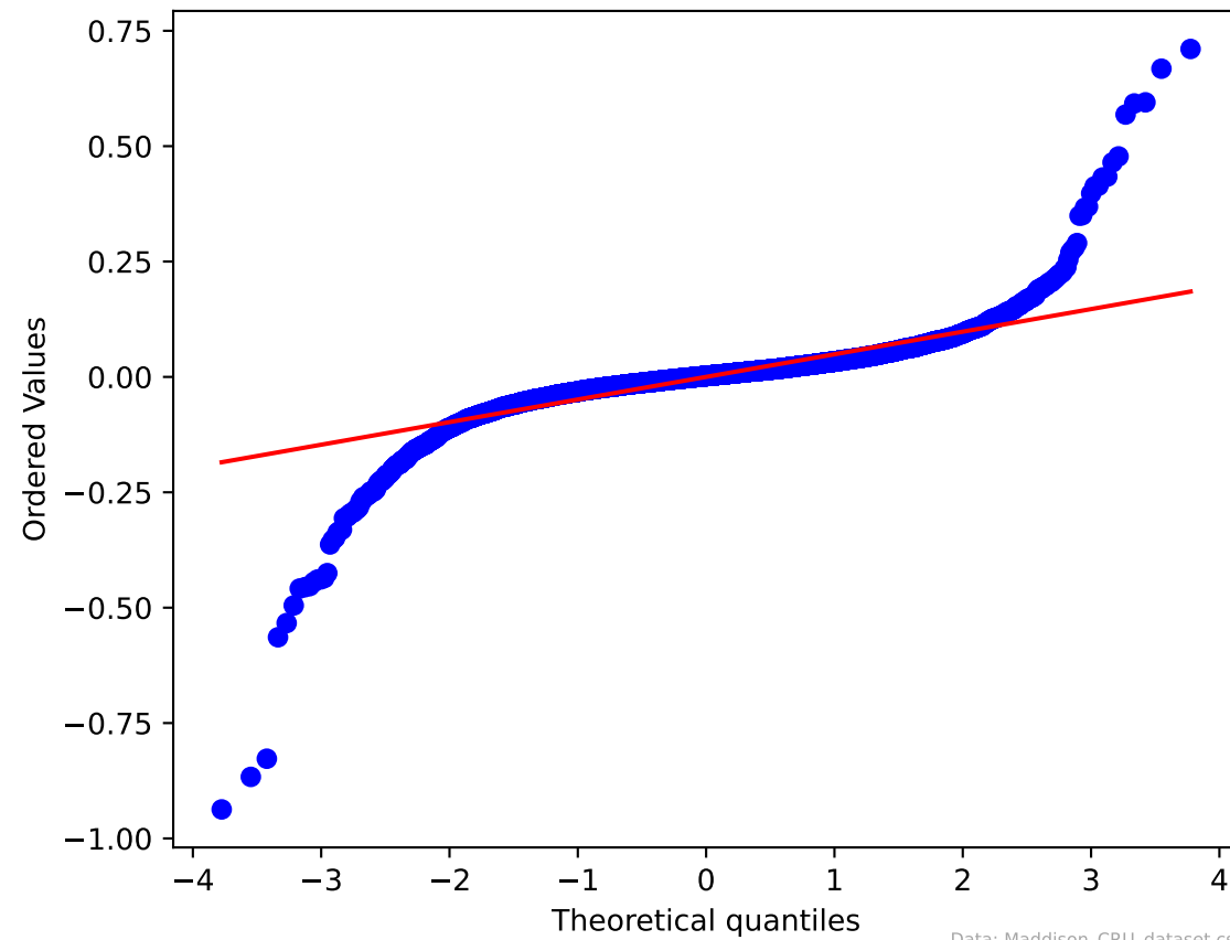
Q-Q Plot
