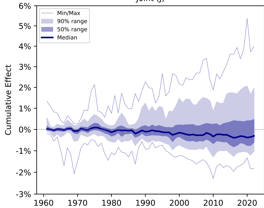
Approach3J Joint (J)
