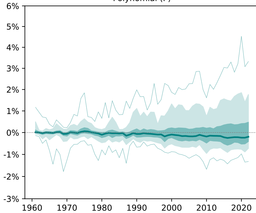
Approach3P Polynomial (P)
