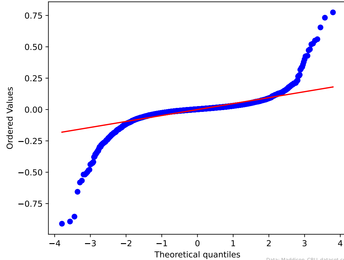
Q-Q Plot
