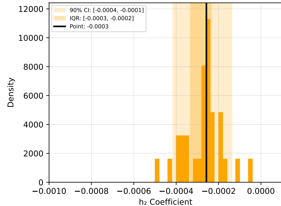
Approach 2: h_2
