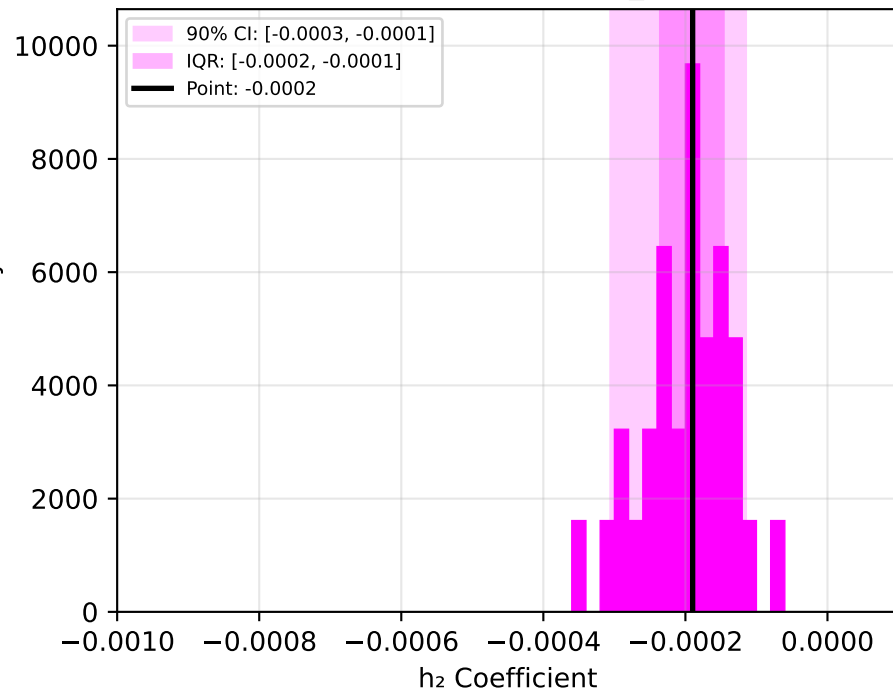
Approach 8: h_2 ( T \leq T_{\text{opt}} )
