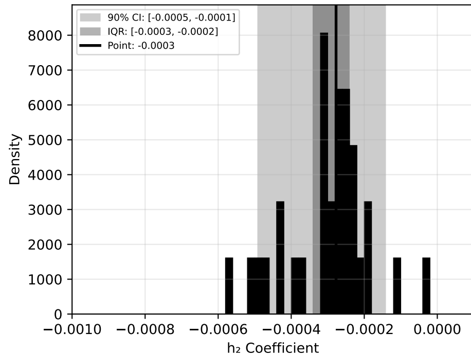
Approach 8: h_2 ( T \leq T_{\text{opt}} )
