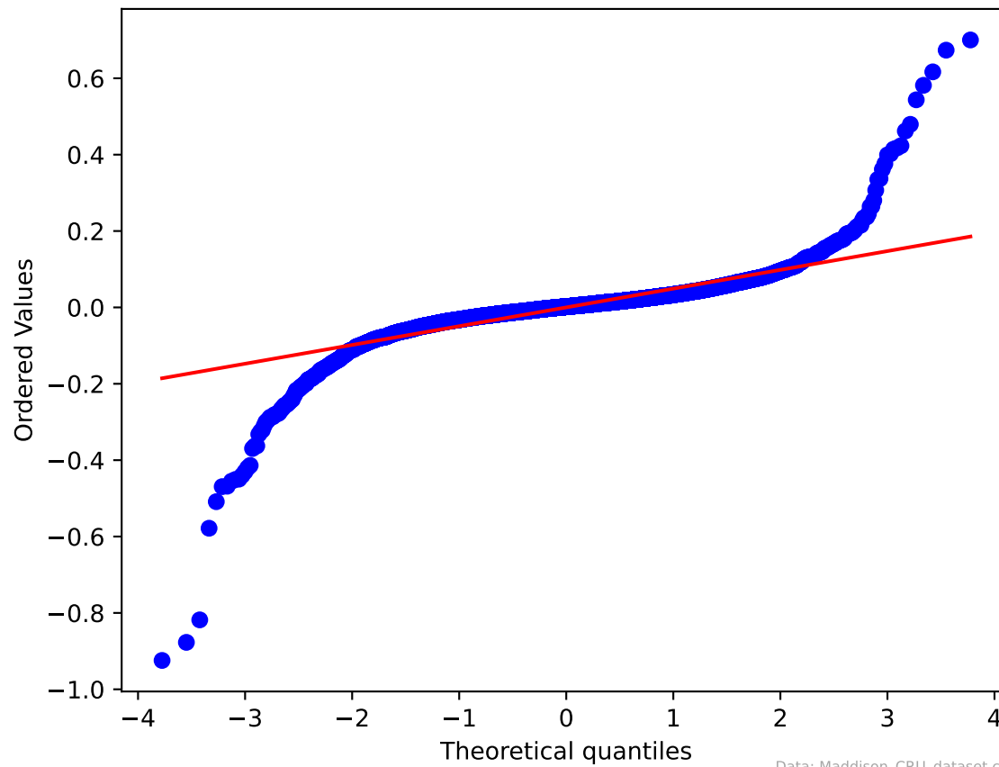
Q-Q Plot
