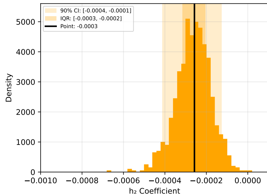
method2: h_2
