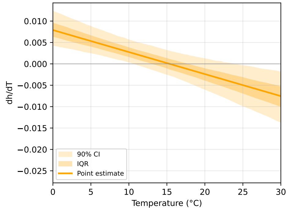
6: Precomputed k LOESS
