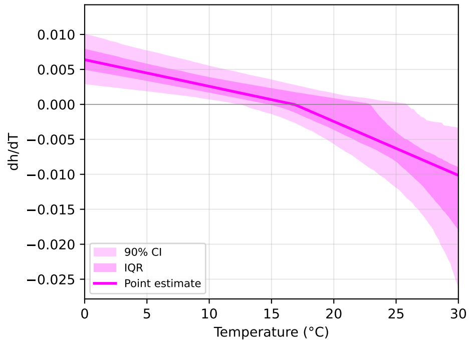
8: Piecewise Quadratic LOESS
