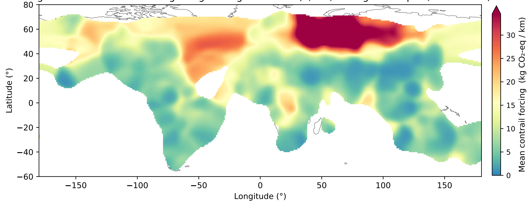
Fig 1b — Mean contrail forcing along flown great-circles (1,000,000 flights sampled, \sigma=3.0 cells)
