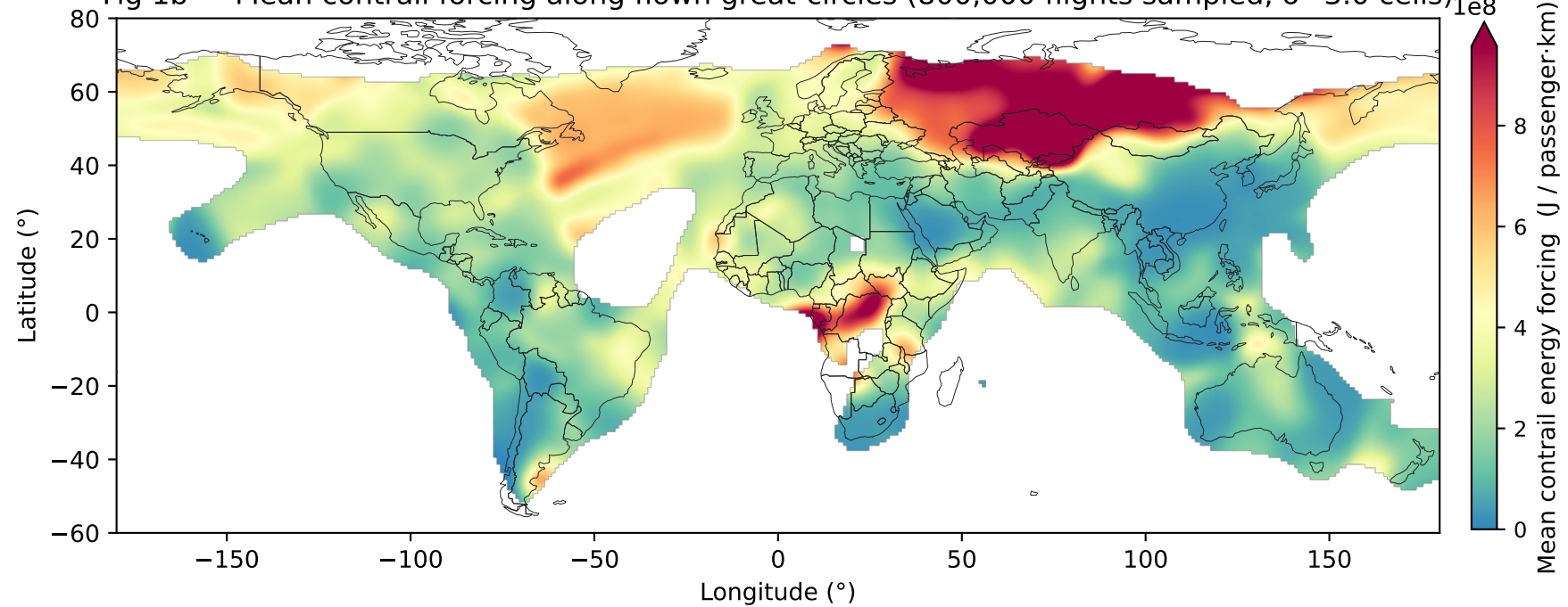
Fig 1b — Mean contrail forcing along flown great-circles (800,000 flights sampled, \sigma=3.0 cells) 1e8
