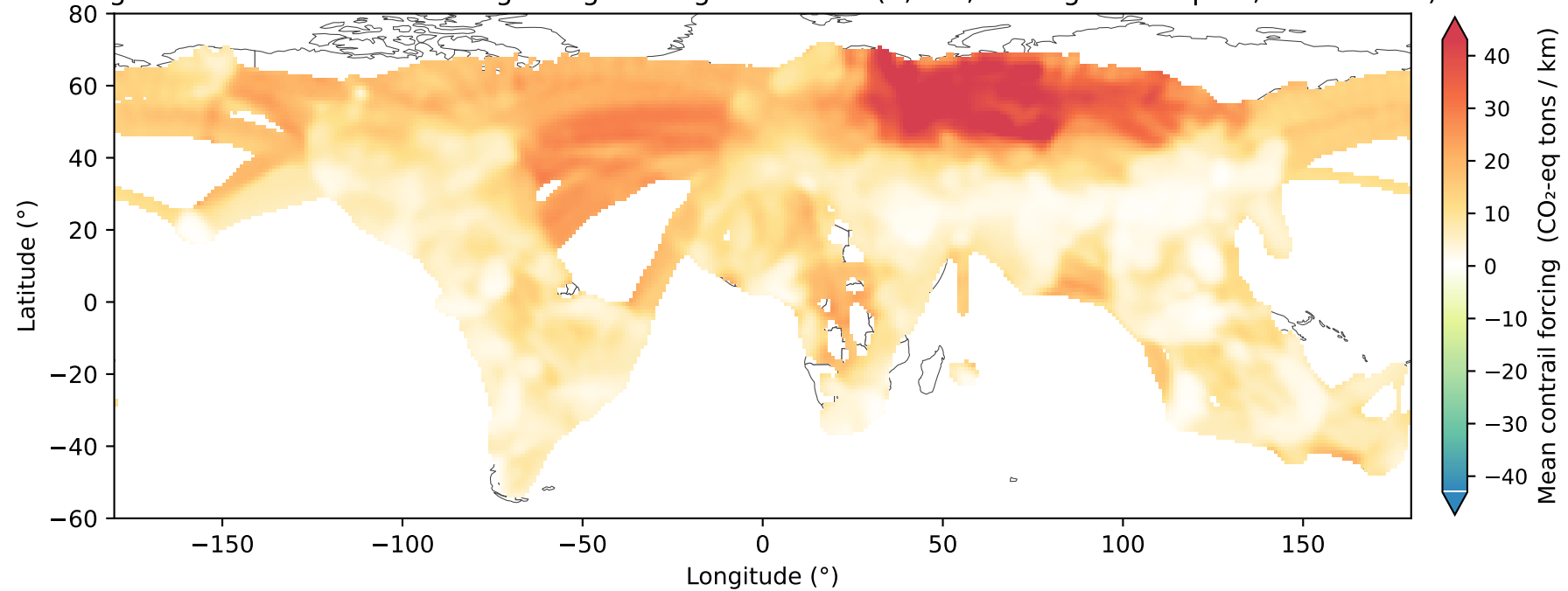
Fig 1b — Mean contrail forcing along flown great-circles (1,000,000 flights sampled, \sigma=1.5 cells)
