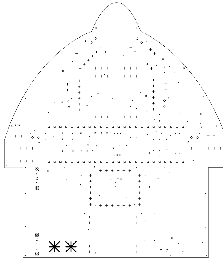
Drill Map:
