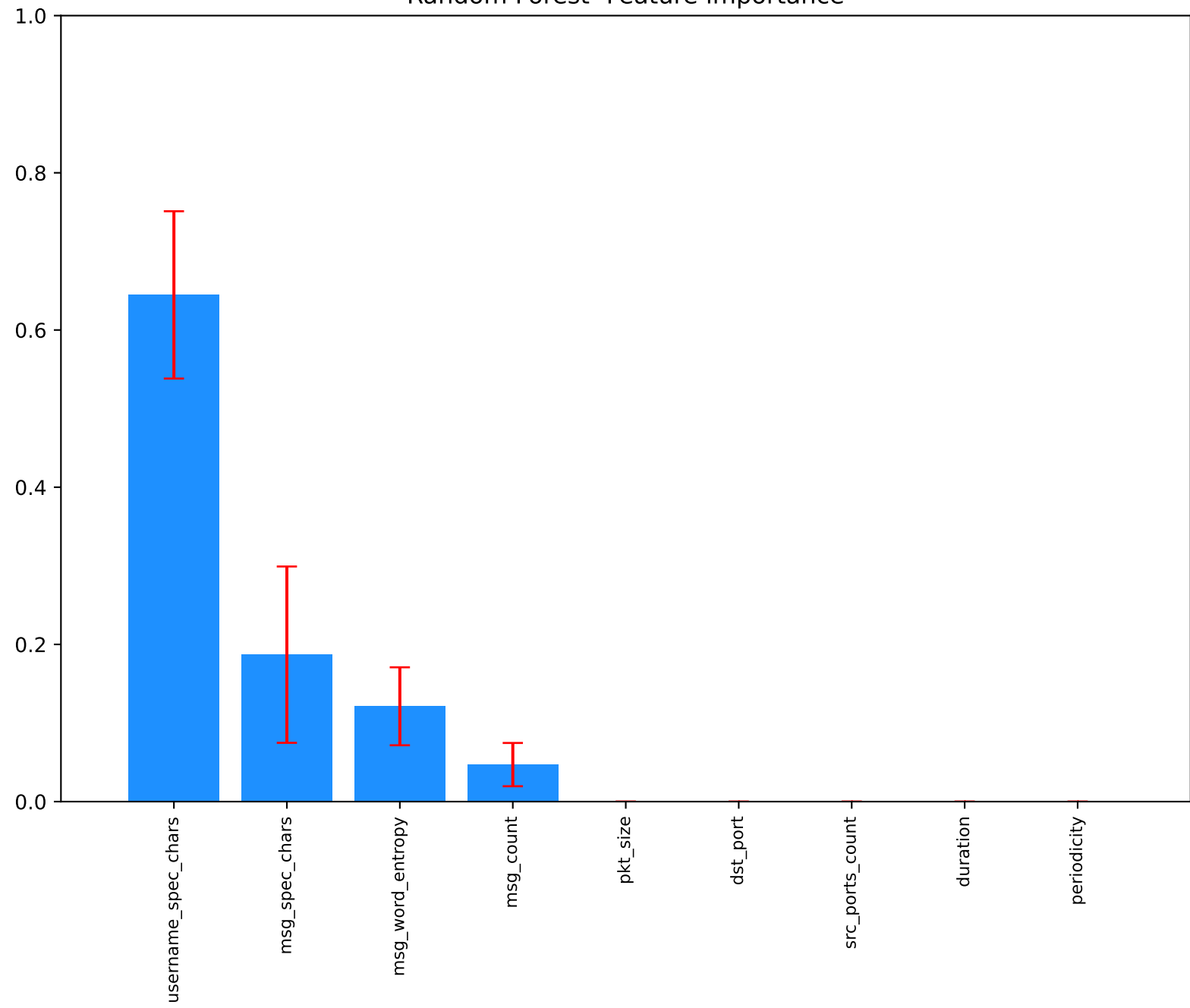
Random Forest- Feature importance
