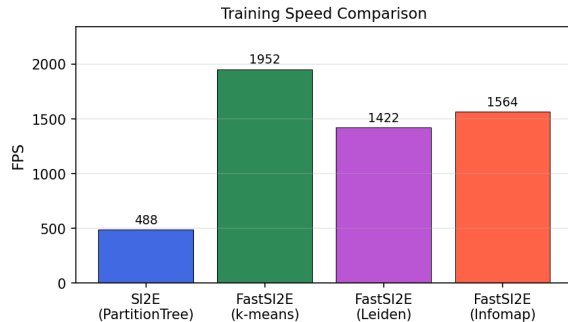
Figure 1: Training throughput (FPS) for SI2E and FastSI2E variants. All fast variants achieve 2.8\text{--}4.0\times speedup over the PartitionTree baseline.
