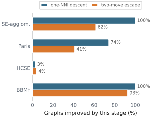
(a) How often each refinement stage helps
