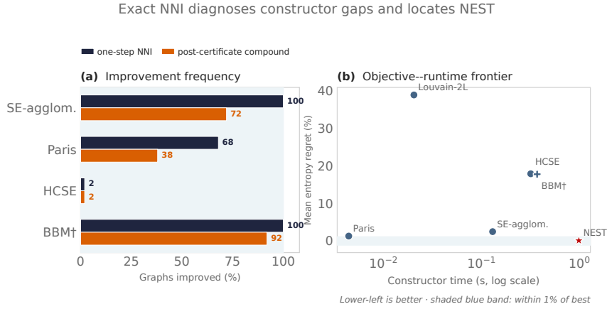
Fig. 3. Operator diagnostics pooled over 50 paired graphs. (a) Fraction of external constructor outputs improved by one-step NNI and by compound search after the one-step certificate. (b) Mean entropy regret versus constructor runtime; lower-left is better. Runtime includes Python allocation tracing and should be interpreted comparatively.
