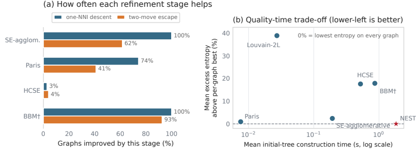
Fig. 3. NNI refinement over 500 graphs. (a) Blue is the fraction of initial trees improved by repeated best-decreasing NNI moves. After no single move helps, the two-move escape may cross one uphill intermediate tree; orange is the fraction whose final endpoint improves further. (b) Each point is an initializer. Excess entropy is 100(H^T - H_{\text{best}}^T)/H_{\text{best}}^T , where H_{\text{best}}^T is the lowest value on the same graph; thus zero is best. The horizontal axis is mean construction time in log seconds, so lower-left is better. Times include Python allocation tracing.
