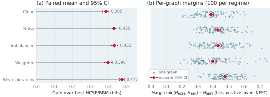
Fig. 2. Paired advantage over external structural-entropy methods. For graph g , the margin is M_g = \min(H_{\text{HCSE},g}^T, H_{\text{BBM},g}^T) - H_{\text{NEST},g}^T , so positive values favor NEST. (a) Regime mean and paired 95% confidence interval. (b) Each blue dot is one of 100 sealed graphs per regime; vertical jitter only separates overlapping dots. Red diamonds are regime means and horizontal whiskers are their 95% confidence intervals. All 500 margins are positive.
