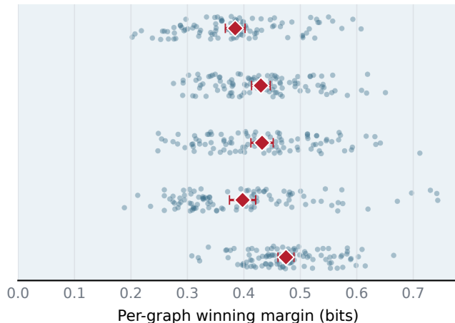
(b) 100 sealed graphs per regime
