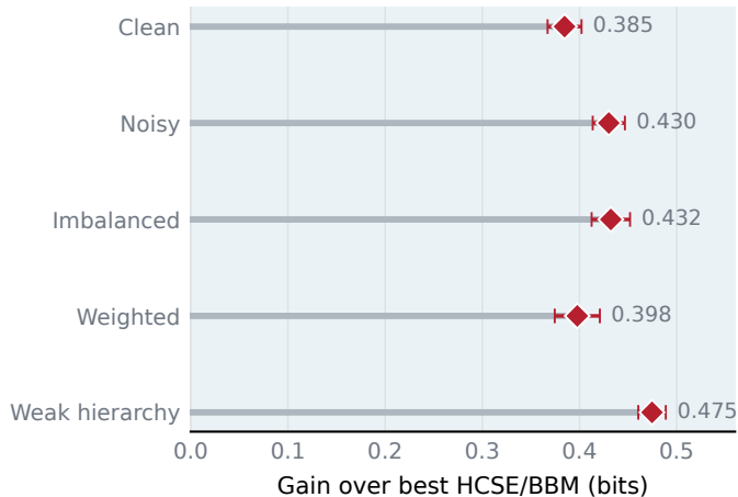
(a) Paired mean and 95% CI
