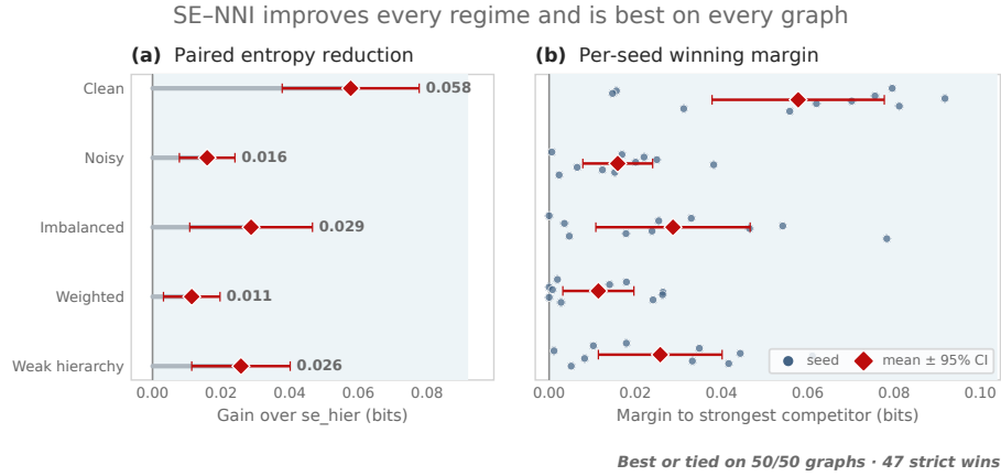
Fig. 2. Paired advantage on the frozen synthetic suite. (a) Reduction relative to se.hier ; diamonds and bars are means and 95% paired confidence intervals. (b) Per-seed margin to the strongest competing method, with small vertical jitter for visibility. SE-NNI is best or tied on all 50 graphs and strictly best on 47.
