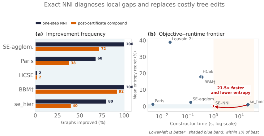
Fig. 3. Operator diagnostics pooled over 50 paired graphs. (a) Fraction of graphs improved by one-step NNI and by compound search after the one-step certificate. (b) Mean entropy regret versus runtime; lower-left is better, and the arrow compares se_hier with SE-NNI. Runtime includes Python allocation tracing and should be interpreted comparatively.
