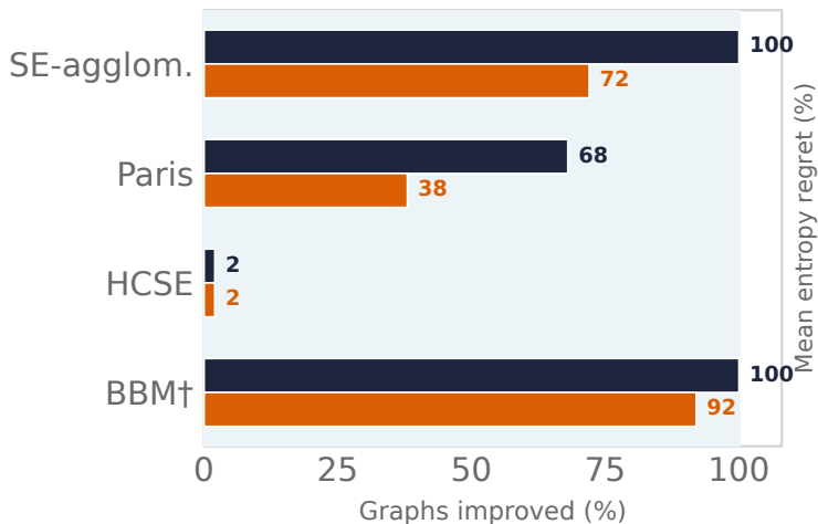
(a) Improvement frequency
