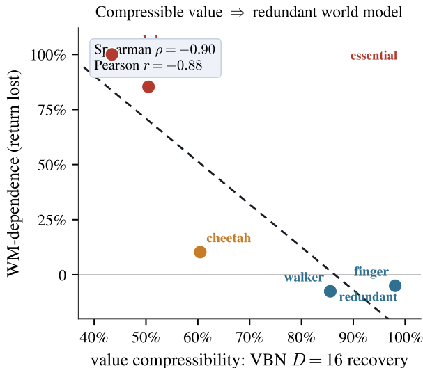
Figure 4: Headline. A single scalar from the VBN probe—return recovered through a D=16 value bottleneck (TD-MPC2)—predicts world-model dependence (Dreamer strip ablation) across five tasks, cross-model. Compressible value \Rightarrow redundant world model. Points for the three remaining collapse tasks (cup-catch, reacher-hard, cart-pole) are being added as their fingerprints complete; the ordering already present here is the diagnostic’s whole claim.
