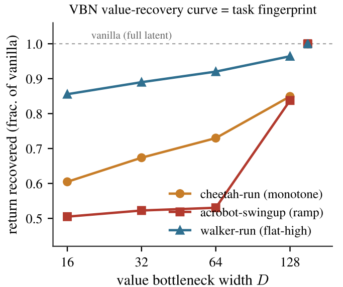
Figure 2: The VBN instrument. Return recovered (fraction of the unbottlenecked agent) as the value head is forced through a width- D bottleneck, TD-MPC2, n=3 seeds. The three shapes are the task fingerprint: WALKER saturates by D=16 (flat-high, highly compressible), CHEETAH keeps climbing (monotone, low compressibility), and ACROBOT ramps late to D^*=128 (needs a large value subspace). Compressibility read off this curve—not the ablation—predicts WM-dependence.
