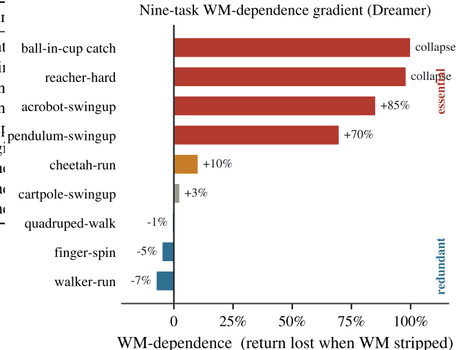
Figure 3: The gradient of Table 1, sorted. World-model value is not a property of the architecture but of the task : it spans near-total collapse (ball-in-cup and reacher-hard score near zero when stripped) to strip-wins (three tasks improve), with a smooth middle. Colour encodes regime; pendulum’s bar is its bimodal n=3 mean (see Table 1).
