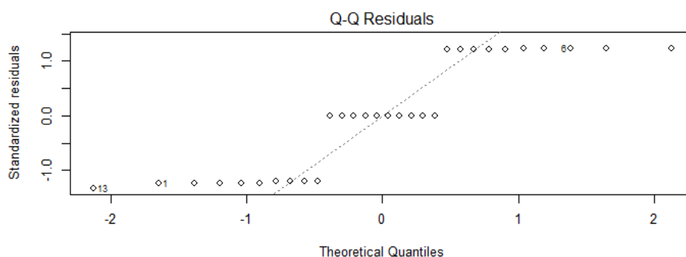
Appendix 13 — Normality of residuals (Q-Q plot)
