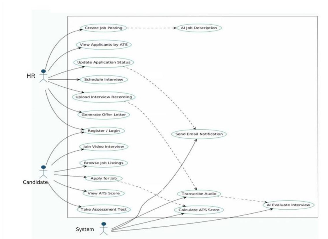
Figure 3.1 Use Case Model
