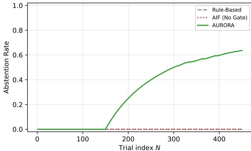
Abstention Rate
