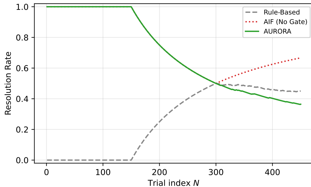
Resolution Rate
