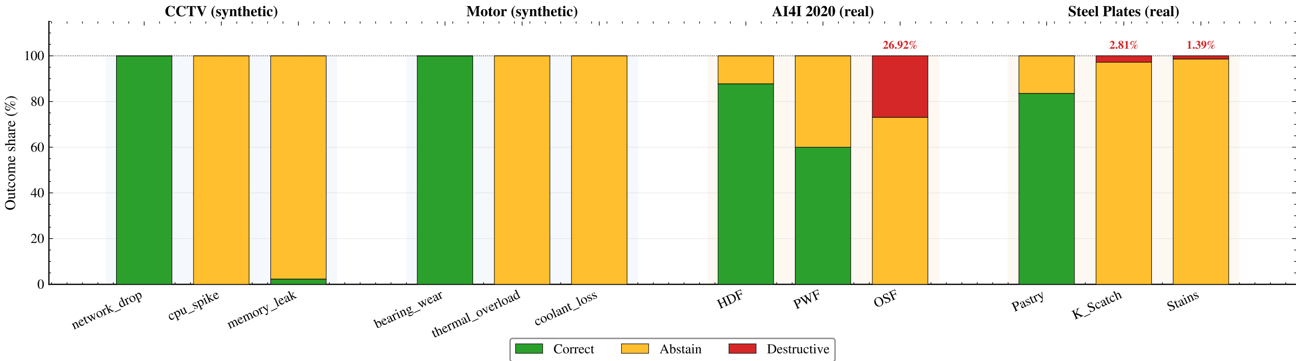
AURORA per-fault outcome composition across four workloads
