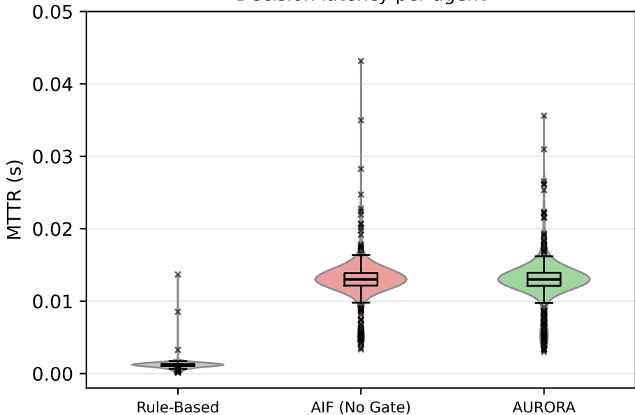
Decision latency per agent
