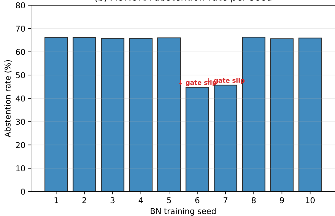
(b) AURORA abstention rate per seed
