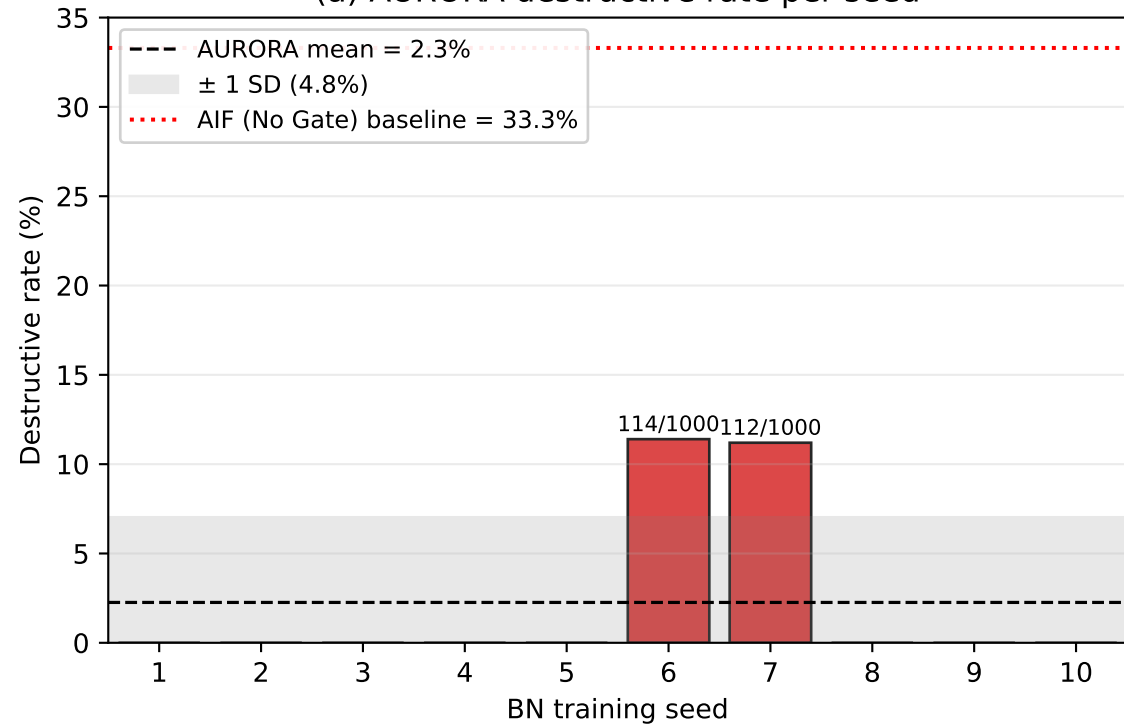
(a) AURORA destructive rate per seed
