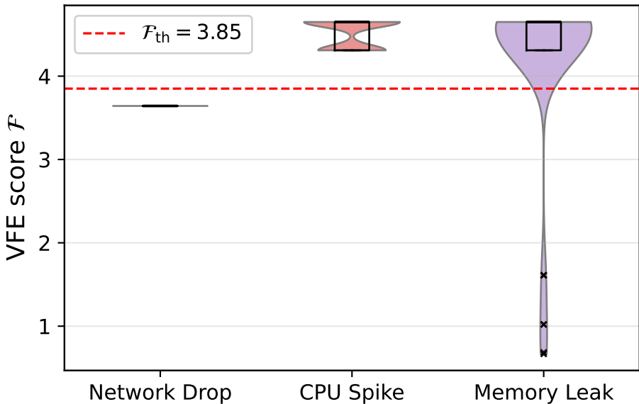
VFE distribution by fault class (AURORA)
