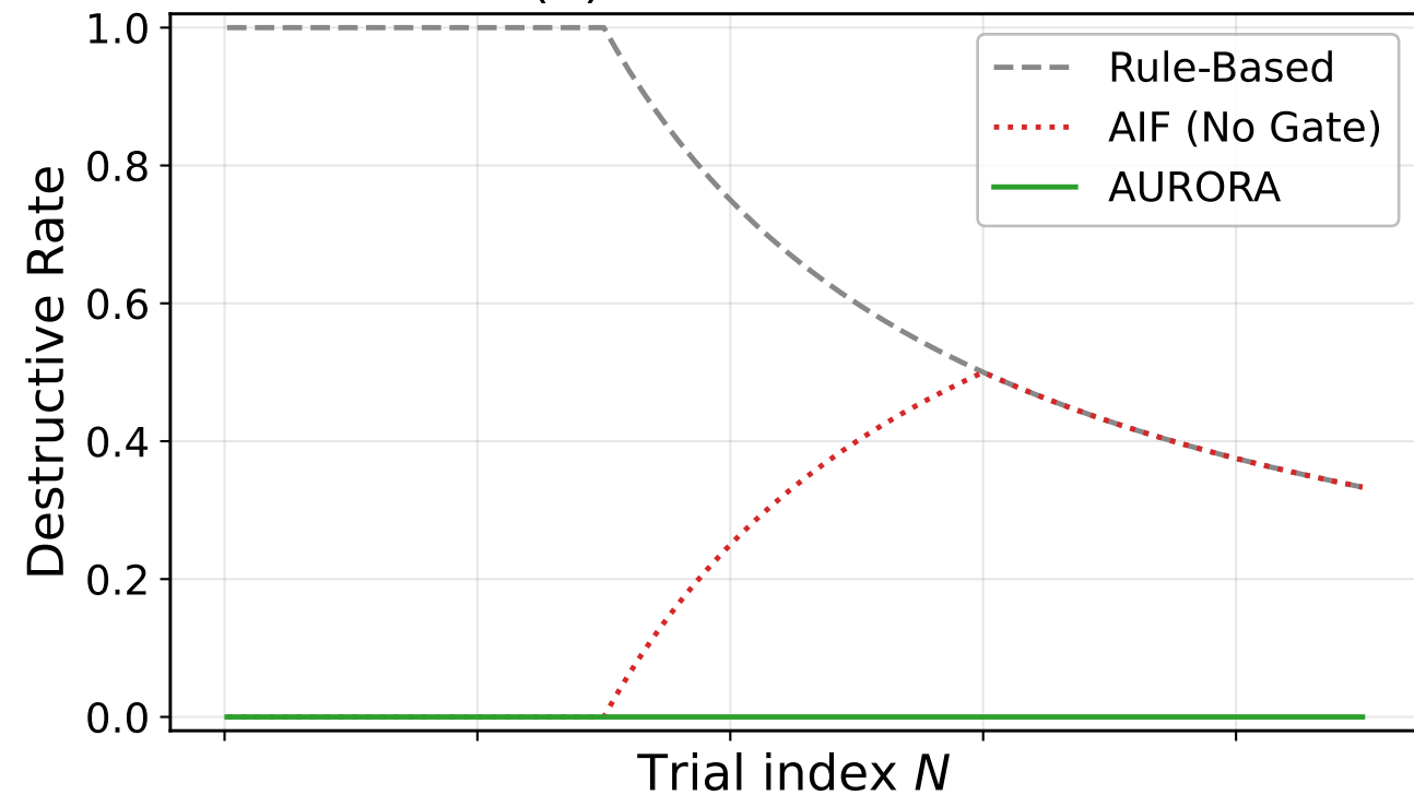
(b) Destructive Rate
