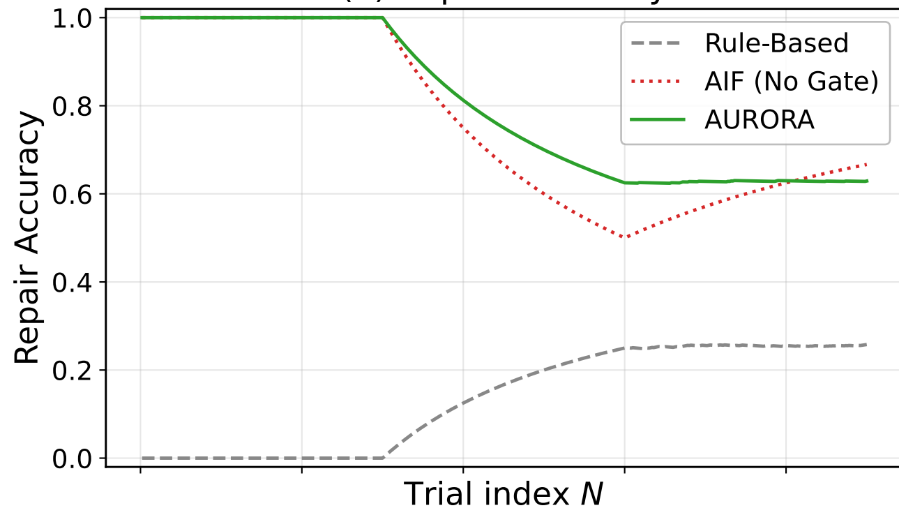
(a) Repair Accuracy
