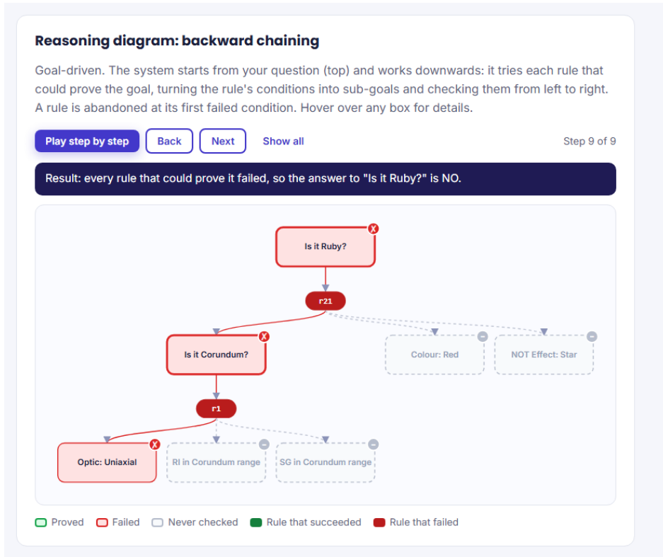
Figure 13. Backward-chaining goal tree for "is it a ruby?" with red spinel data
