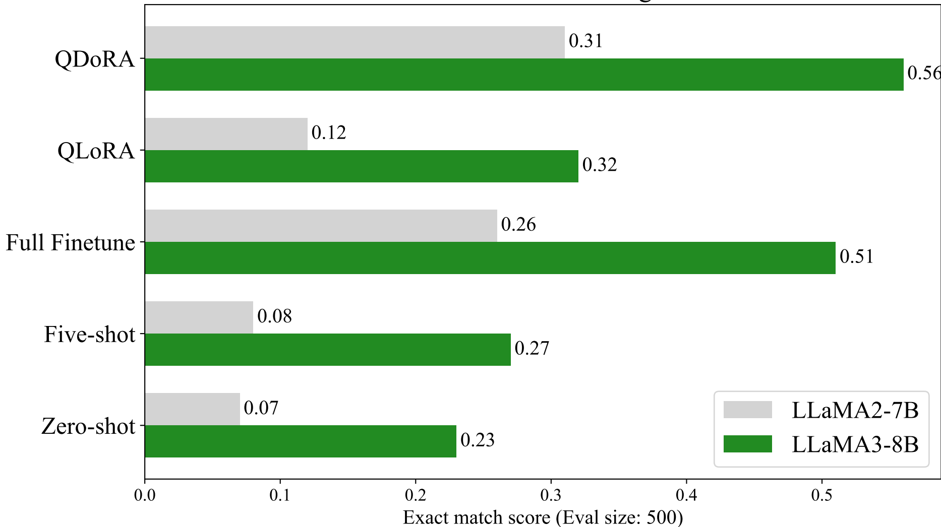
100k Orca-Math finetuning results
