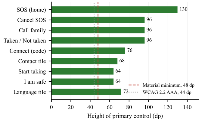
Fig. 4. Height of the primary control on each elder screen, parsed from source. Every primary control exceeds the 48 dp platform minimum and the 44 dp WCAG 2.2 AAA target-size criterion; the median is 76 dp and the emergency control is 130 dp.
