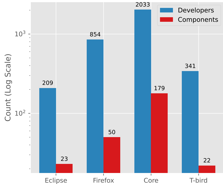
Candidate Pool &amp; Component Granularity
