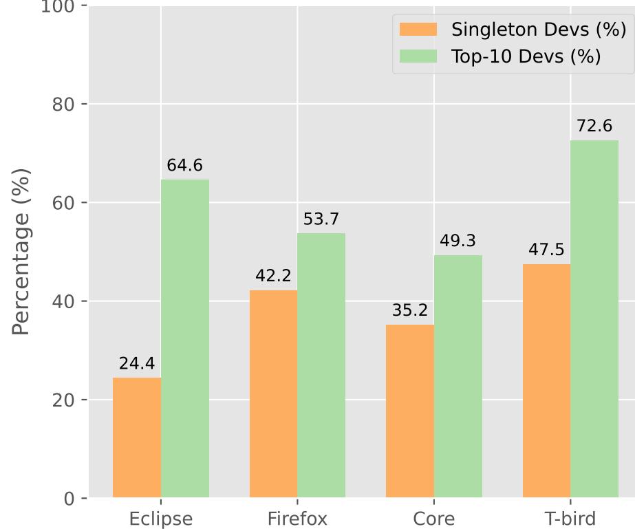
Sparsity &amp; Concentration
