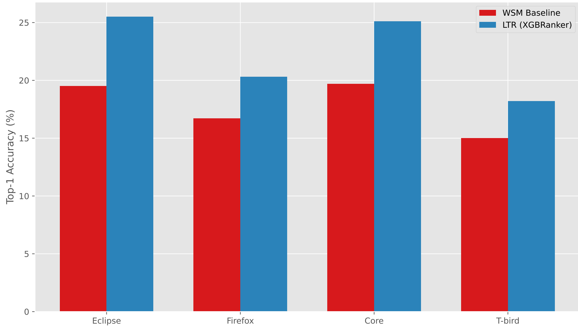
Top-1 Accuracy Comparison: WSM vs LTR
