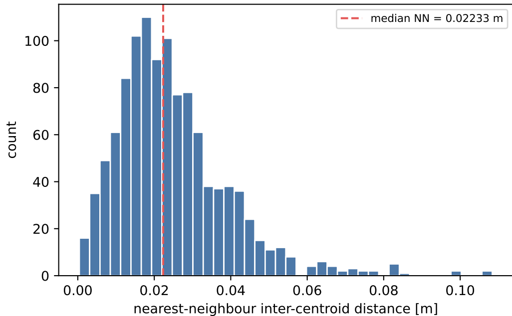
Lift/image: distances the kernel must resolve n=1118 (1224 clusters, 558 rounds)
