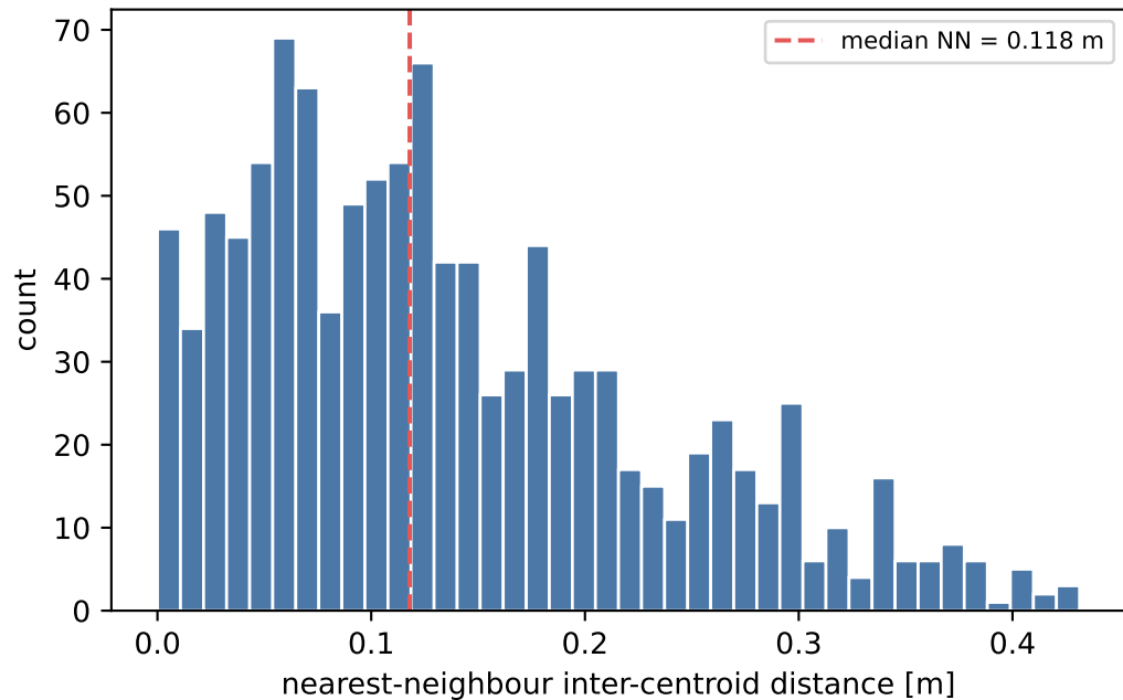
PushT/state: distances the kernel must resolve n=1096 (1096 clusters, 413 rounds)
