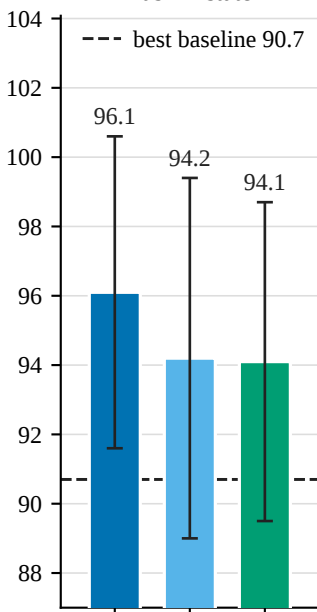
Push-T state
