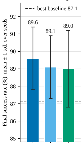
GridWorld image
