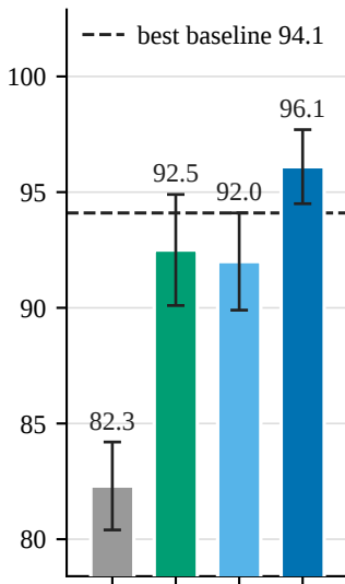
Push-T state
