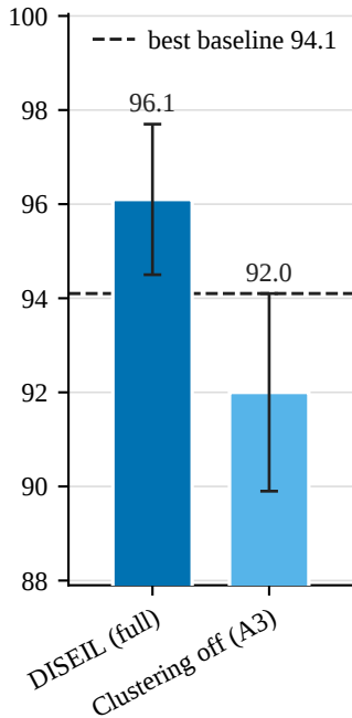
Push-T state
