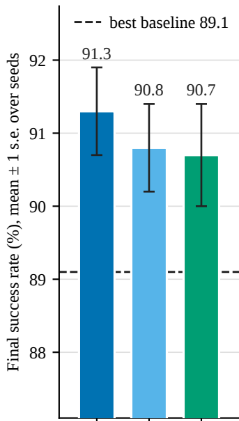
GridWorld image
