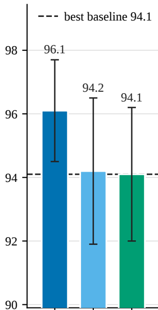
Push-T state
