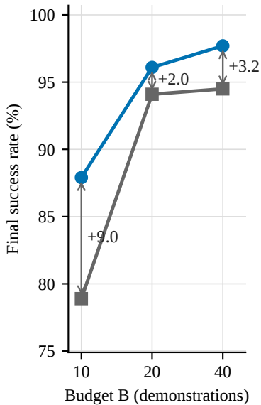
Push-T state
