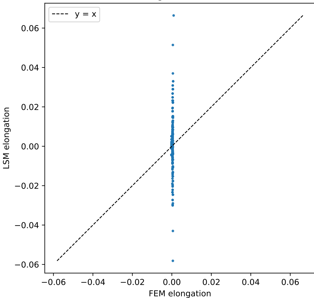
Bond elongation: LSM vs FEM
