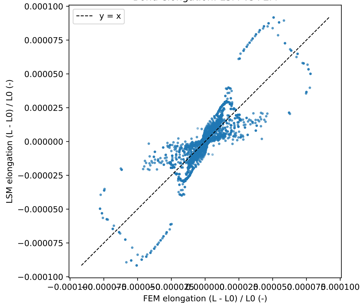
Bond elongation: LSM vs FEM
